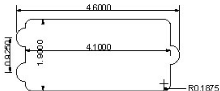
MM5.2, MM5.3, MM5.4 wide cover (available with various pole spacings)
